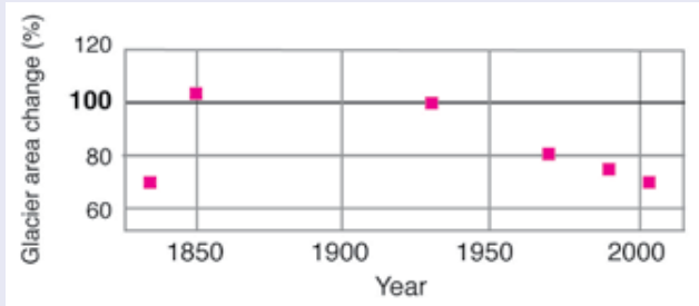
Figure 5.9: Extent (%) of the total surface area of glaciers of the tropical Cordillera Blanca, Peru, relative to their extent around 1925 (=100) (Georges, 2004). The area of glacier in the Cordillera Blanca in 1990 was 620 km 2 . [Extracted from WGI Figure 4.16]
